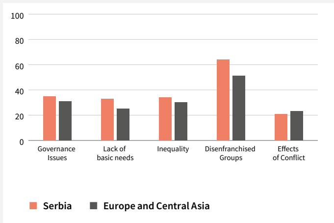
Figure 3. Vulnerability of Serbia to modern slavery by dimension of vulnerability, compared to the regional average
